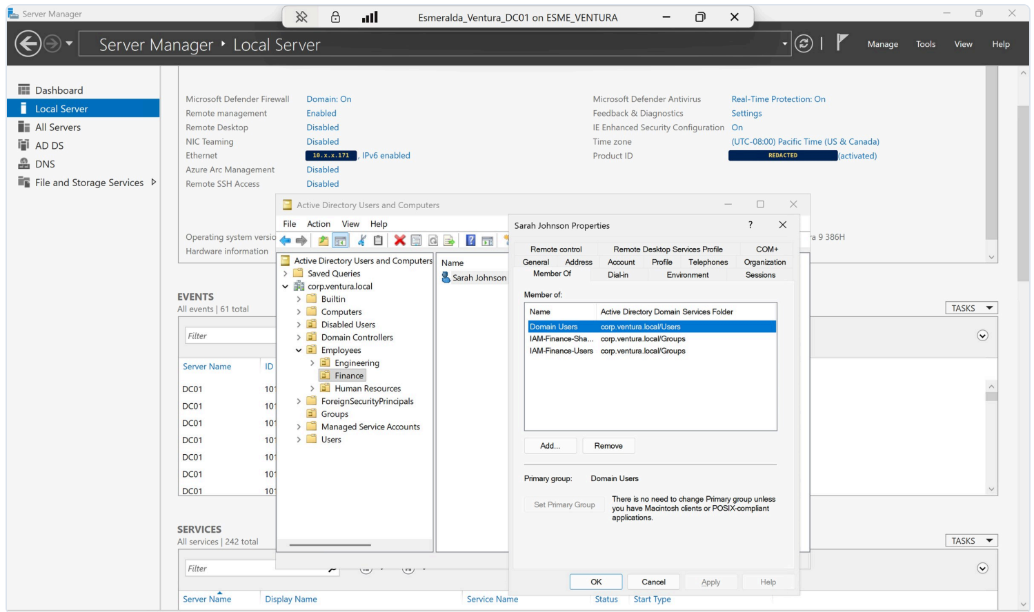
Figure 13. Member Of tab: Domain Users, IAM-Finance-SharedDrive and IAM-Finance-Users.
