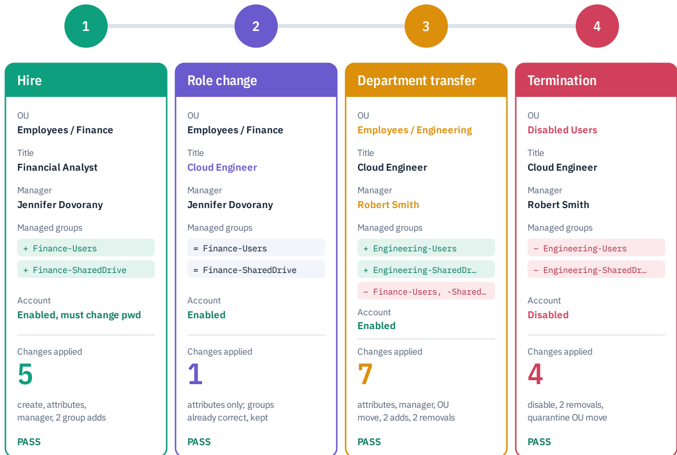
Figure 10. Sarah Johnson's state after each run. Colored values show what changed at that step. Group names drop the IAM- prefix for space.
