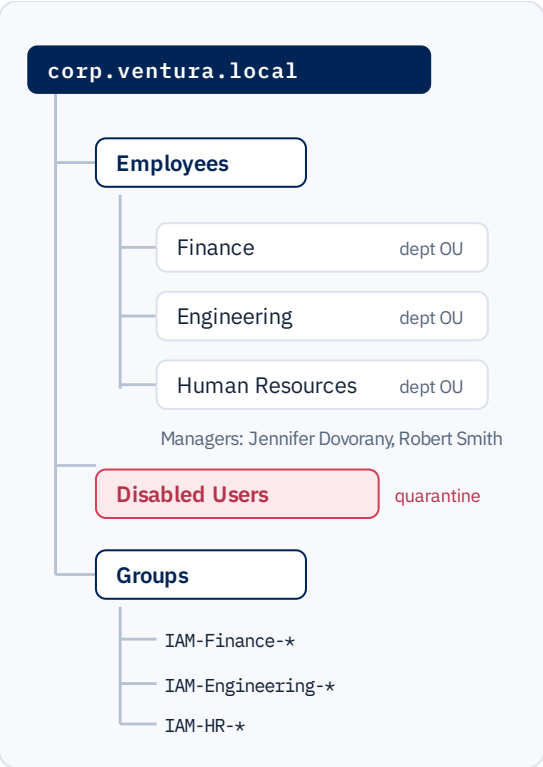
Figure 3. OU design. Department OUs mirror HR departments, and all OUs are protected from accidental deletion.
