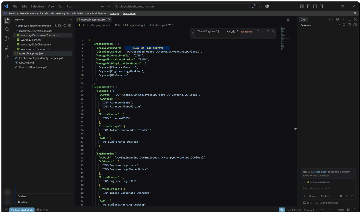
Figure 6. AccessMappings.json : organization settings (quarantine OU, IAM - prefix, AVD application groups) and the Finance and Engineering department baselines. The initial password is redacted.
