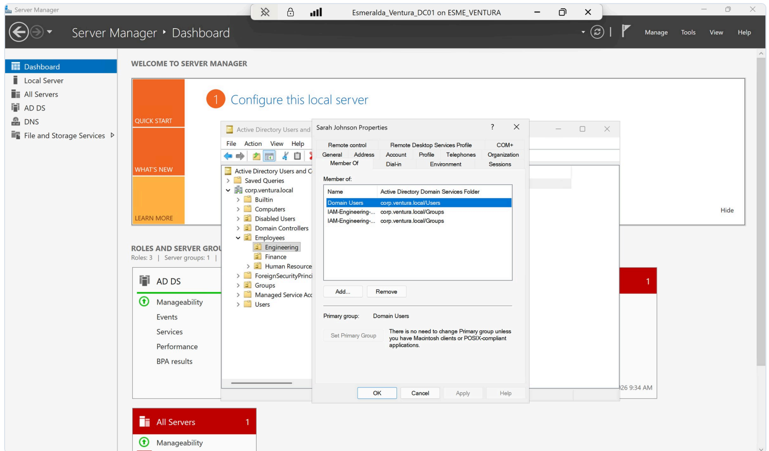
Figure 18. Member Of after the transfer: Domain Users , IAM-Engineering-SharedDrive and IAM-Engineering-Users . No Finance access remains.
