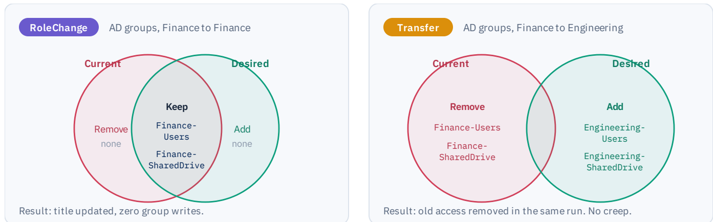
Figure 5. Set reconciliation using real test data. Groups without the IAM- prefix, such as Domain Users, are filtered out before comparison and never touched.
