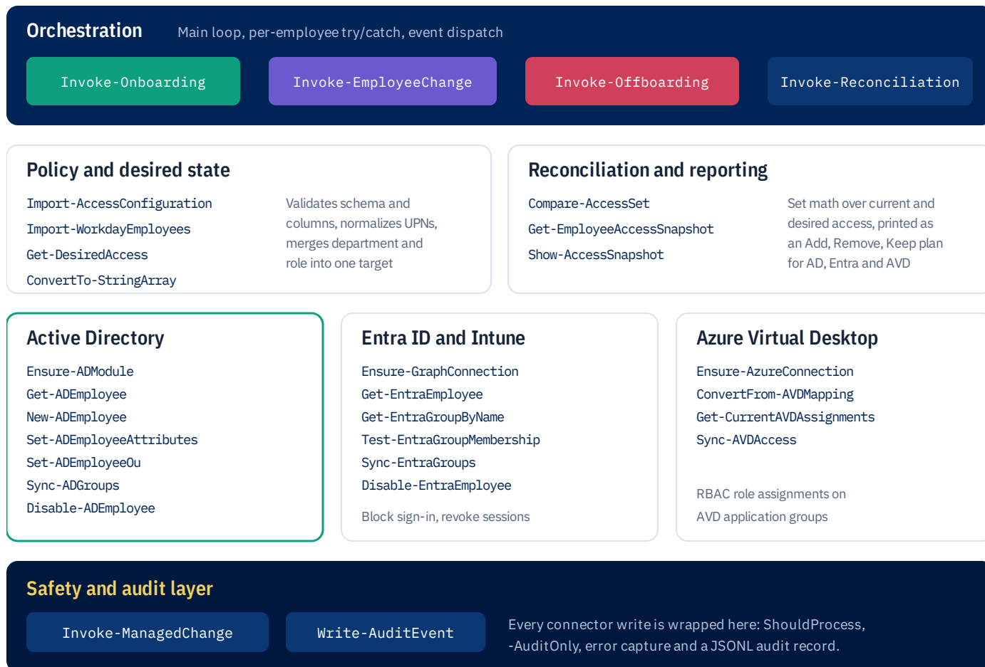
Figure 4. Function map of Invoke-EmployeeIdentityLifecycle.ps1 , showing all 30 functions grouped by layer.
