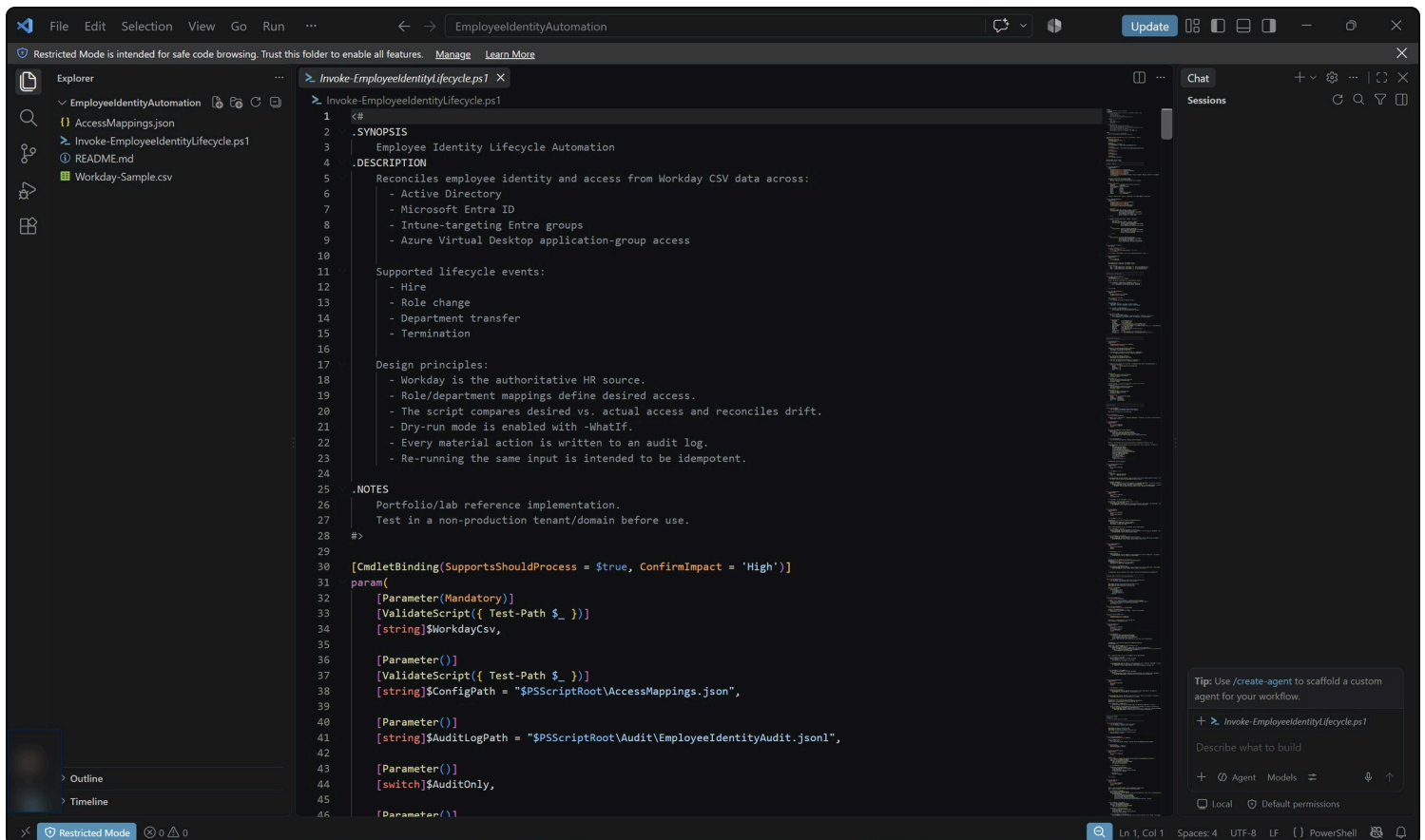
Figure 7. Invoke-EmployeeIdentityLifecycle.ps1 : comment-based help listing the design principles, and the CmdletBinding(SupportsShouldProcess = $true, ConfirmImpact = 'High') parameter block.
